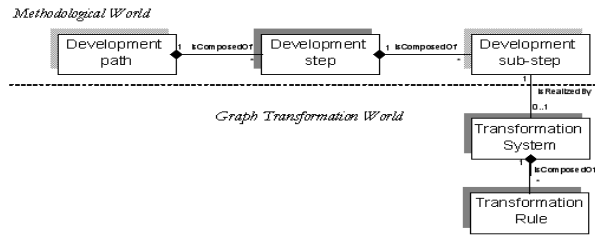
Fig. 1. Articulation of graph transformations with transformational development of UIs
