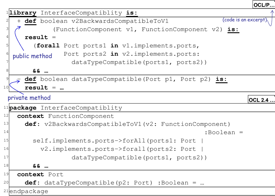
Fig. 4: Example for an OCL library with public and private query functions
