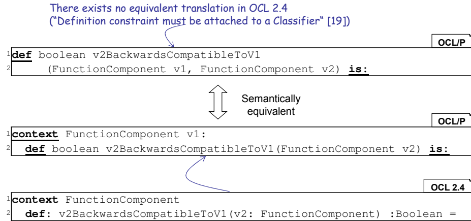
Fig. 5: Example for OCL def operator in non-member syntax
