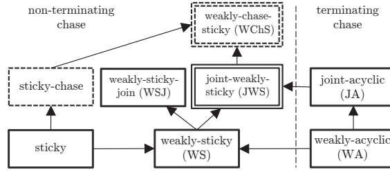
Fig. 2. Generalization relationships among program classes.
