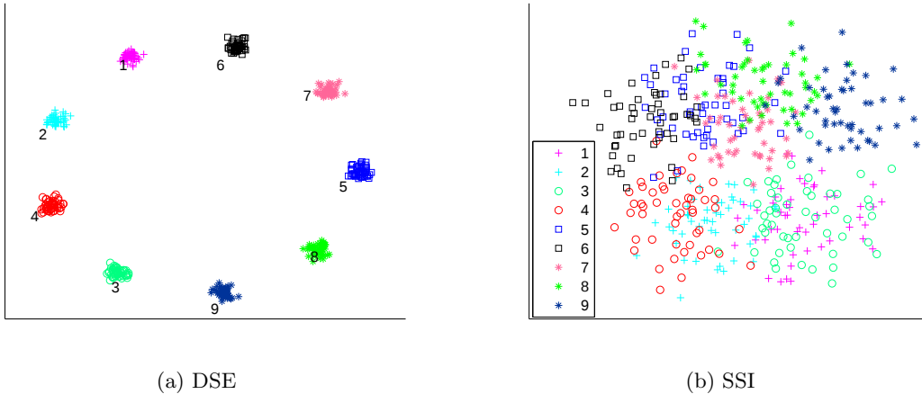
Figure 1: Embeddings of the NIPS papers with the dimensionality C = 2 , produced by DSE and SSI using 40% distinct positive links for training. The section numbers of the papers are shown as well.
