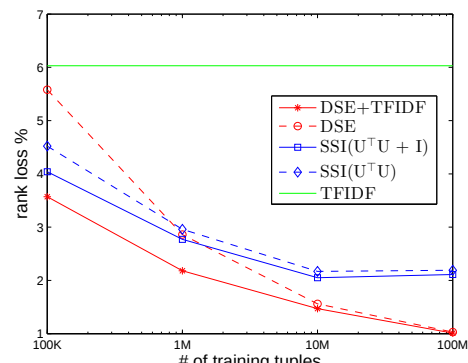
Figure 2: Test results using top 1000 most frequent words.
